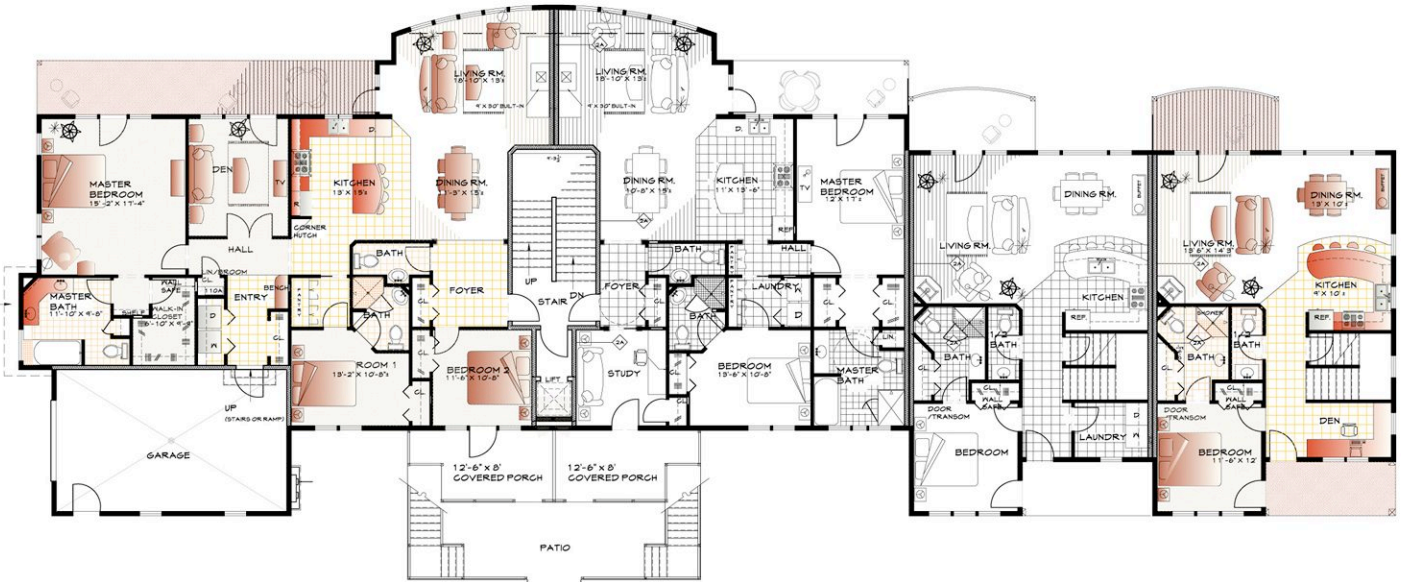
MAIN LEVEL PLAN SF = 6,051 ±
